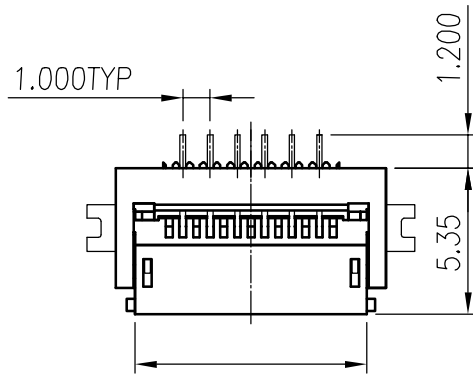
Connector outline
