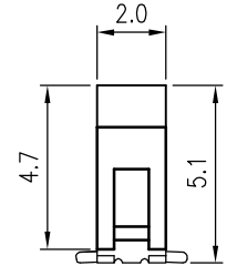
NO. OF CONTACTS 15 PIN~30 PIN
