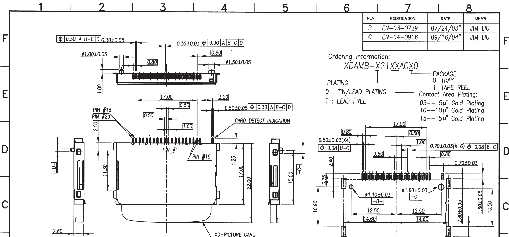
PCB LAYOUT TOP VIEW
