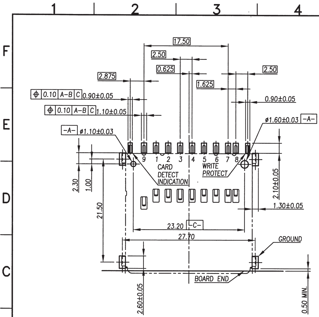
PC BOARD LAYOUT COMPONENT SIDE
