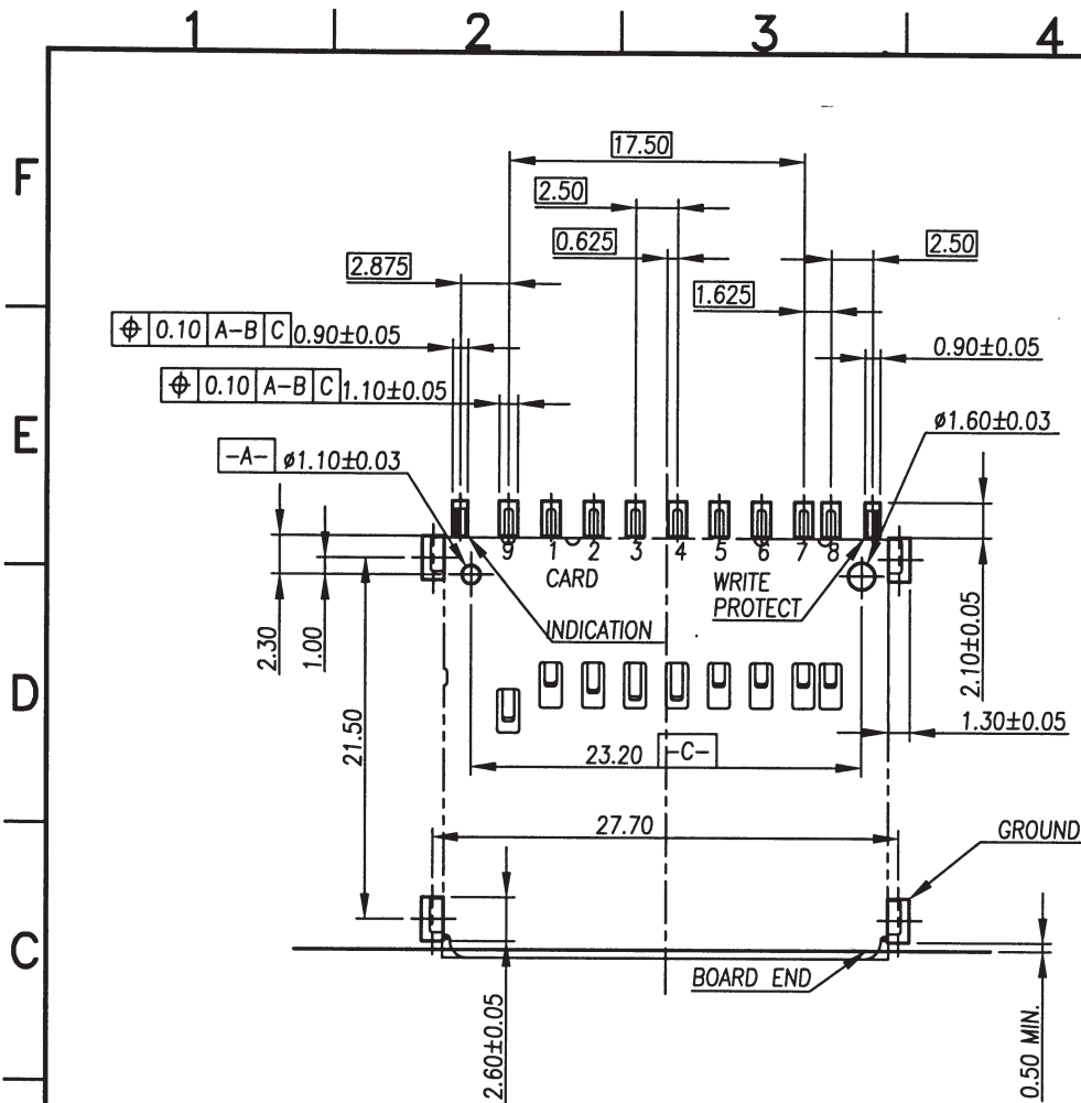
PC BOARD LAYOUT COMPONENT SIDE
