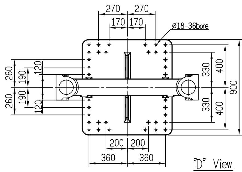
Moving platen and ejection
