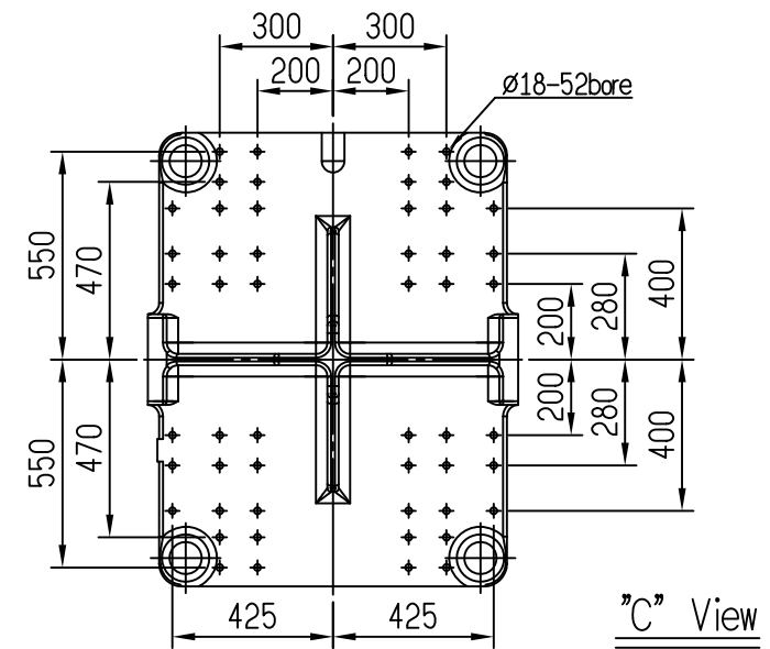
Fixed platen and ejection
